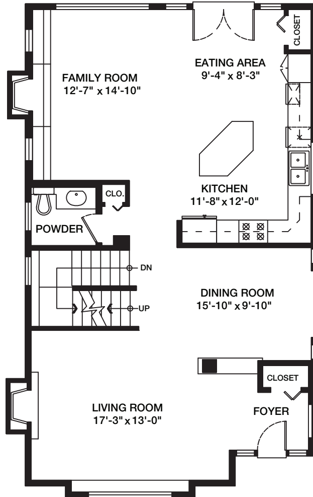
Main Floor Plan Floor Area: 1,045 sq.ft.
