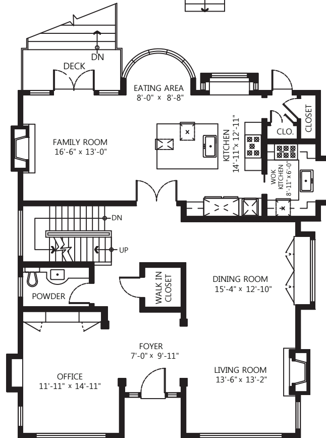
MAIN FLOOR PLAN Floor Area: 1,532 sq.ft. Ceiling Height: 9'-8"
