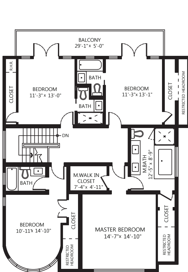
UPPER FLOOR PLAN Floor Area: 1,395 sq.ft. Peak Ceiling Height: 11'-9"
