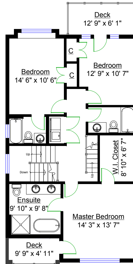
UPPER LEVEL Ceiling Height = 8' 1"
