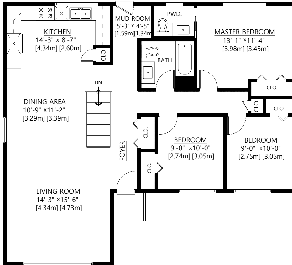
Main Floor Plan Floor Area: 1,206 sq.ft. Floor Area: 112.04 sq.m.
