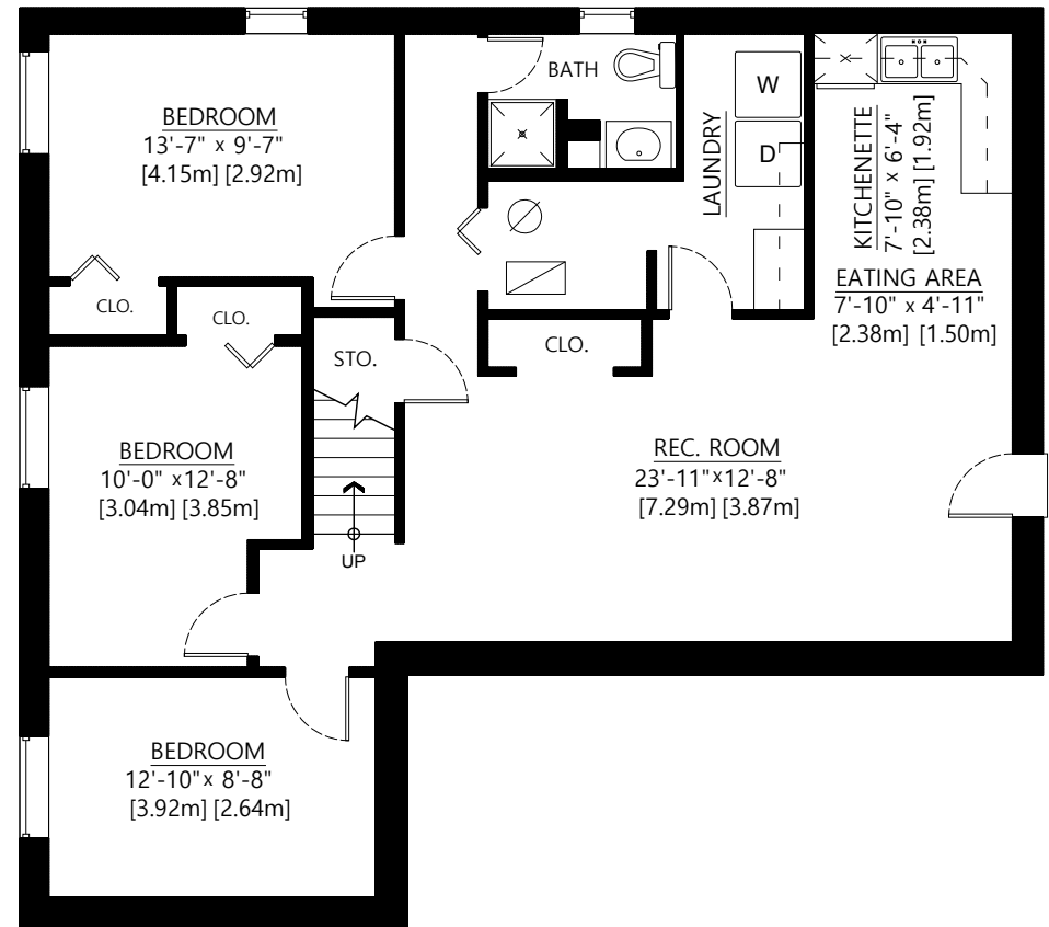
Below Grade Floor Plan Floor Area: 1,034 sq.ft. Floor Area: 96.06 sq.m.
