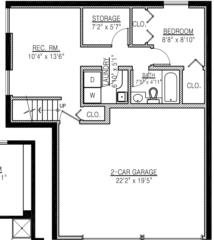
LOWER FLOOR PLAN FLOOR AREA: 546 sq. ft.
