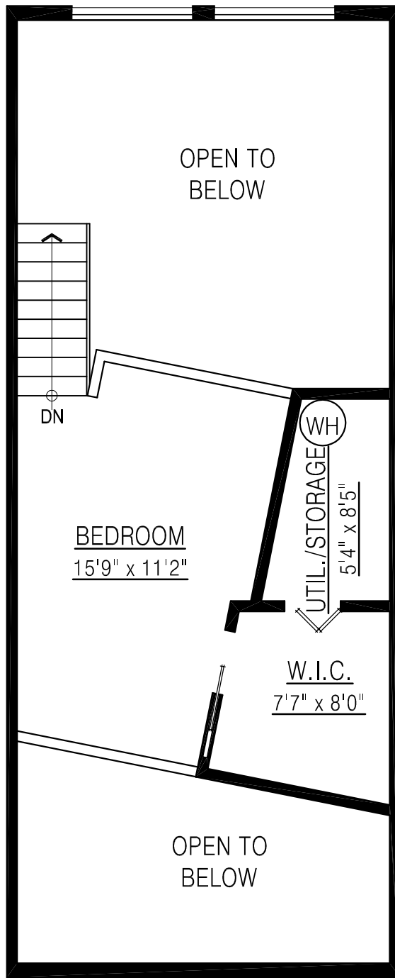
UPPER FLOOR PLAN FLOOR AREA: 294 sq. ft.
