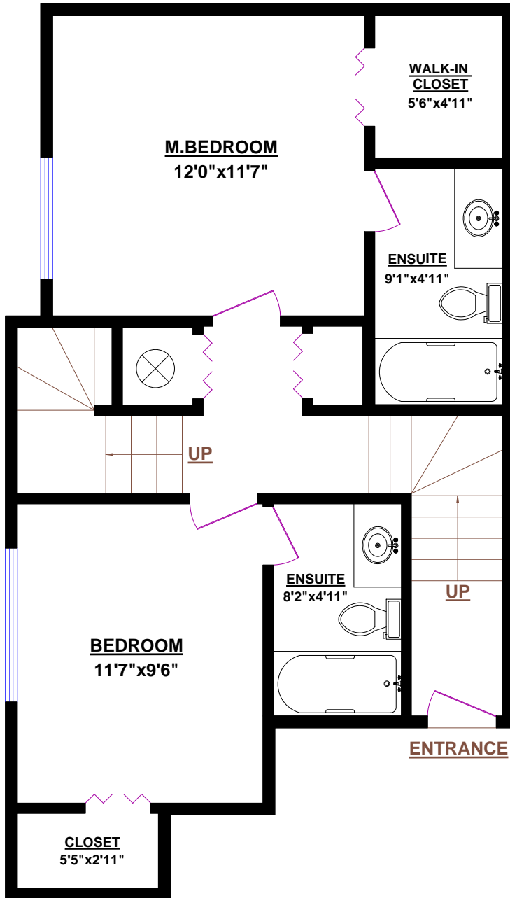
LOWER LEVEL
