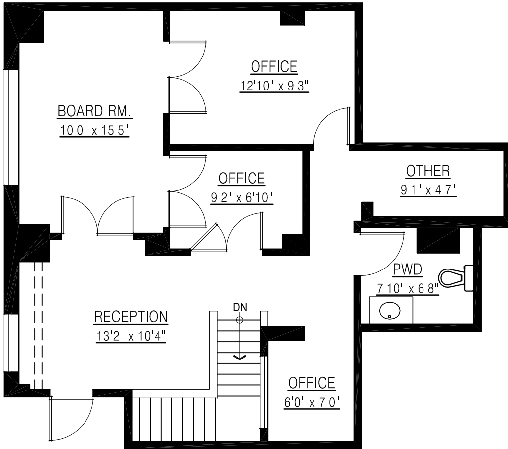
MAIN FLOOR PLAN FLOOR AREA: 777 sq.ft.
