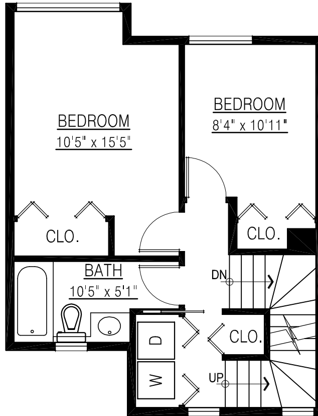
UPPER FLOOR PLAN FLOOR AREA: 465 sq.ft.
