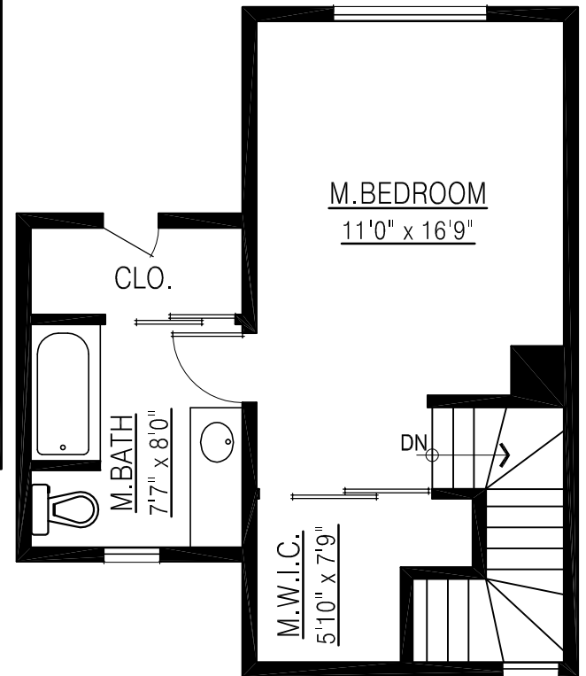
TOP FLOOR PLAN FLOOR AREA: 388 sq.ft.
