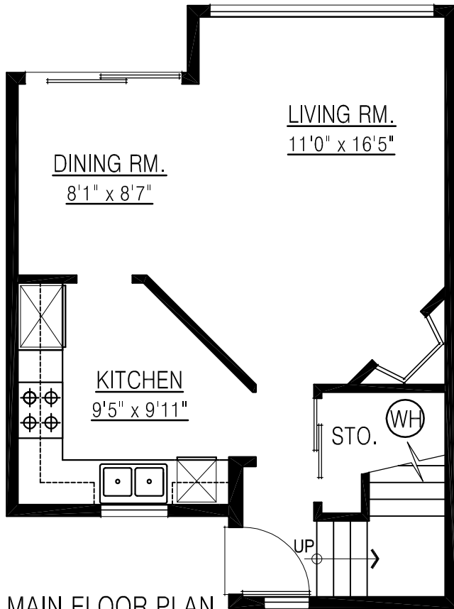
MAIN FLOOR PLAN FLOOR AREA: 476 sq.ft.
