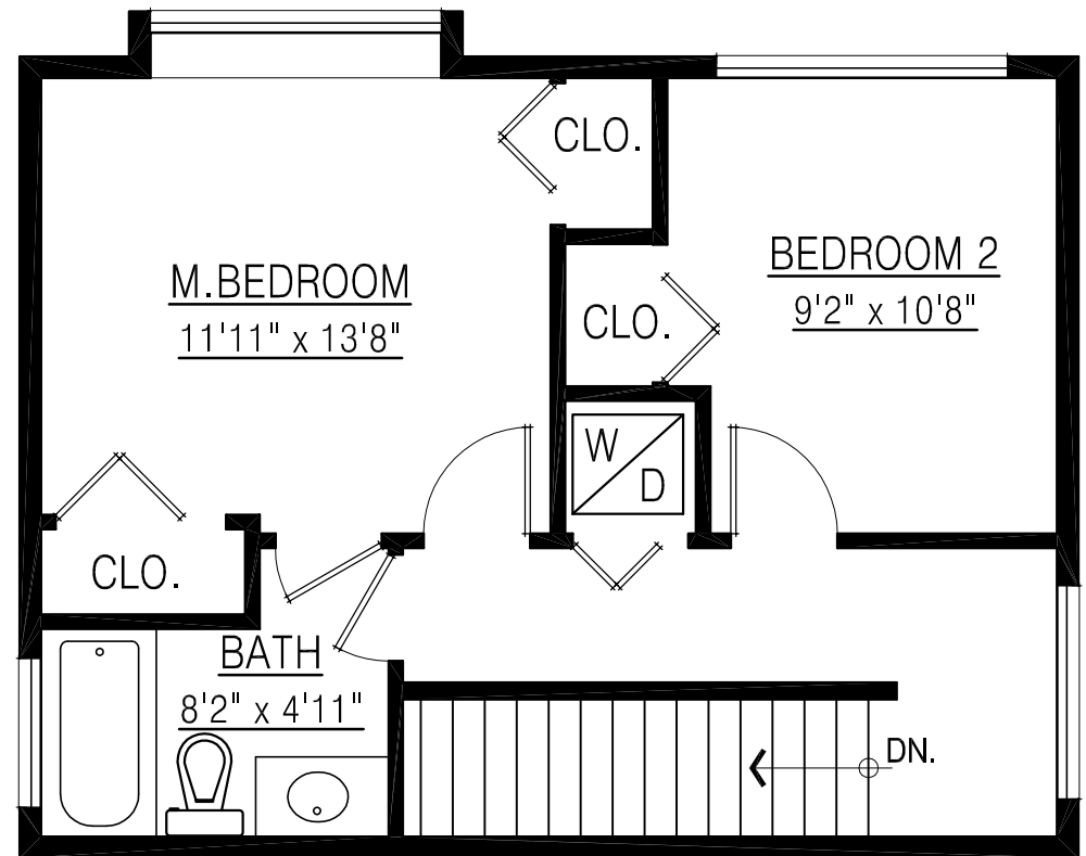
UPPER FLOOR PLAN FLOOR AREA: 432 sq. ft.
