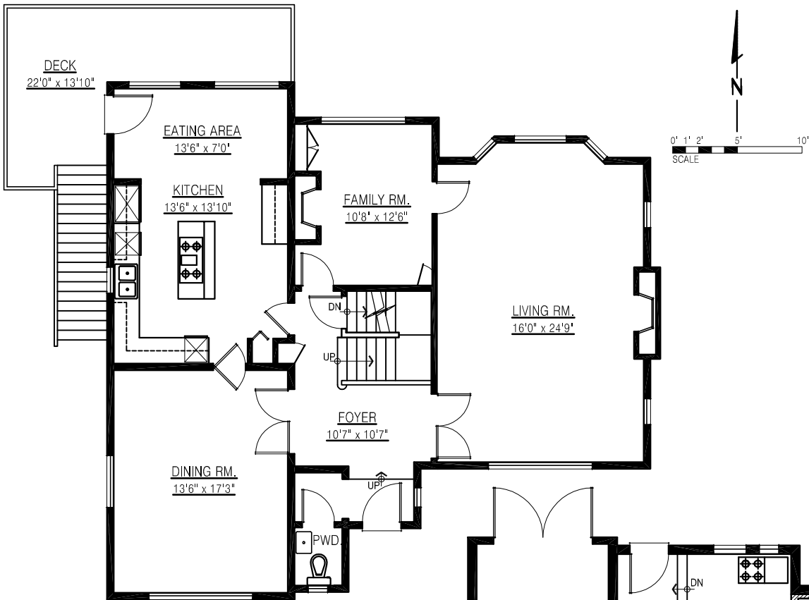
MAIN FLOOR PLAN FLOOR AREA: 1,356 sq.ft.
