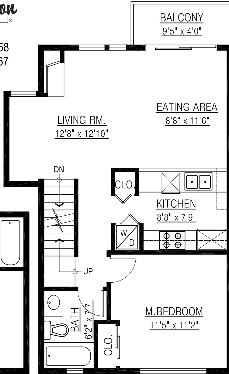
UPPER FLOOR PLAN FLOOR AREA: 628 sq.ft.
