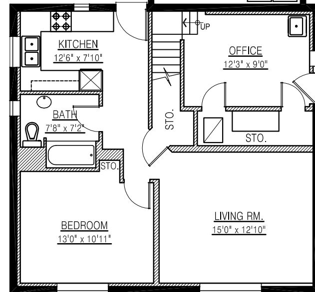
LOWER FLOOR PLAN FLOOR AREA: 852 sq.ft.
