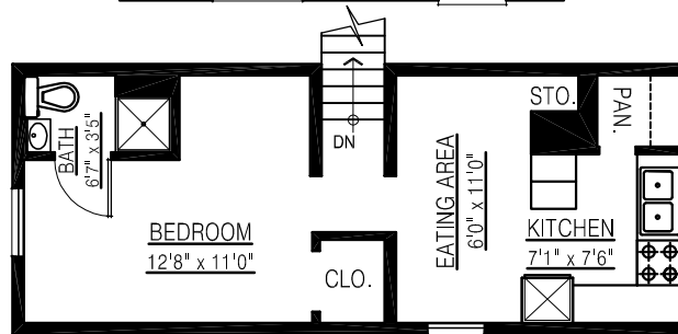
UPPER FLOOR PLAN FLOOR AREA: 356 sq.ft.
