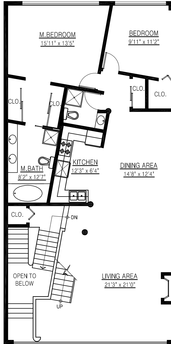
MAIN FLOOR PLAN FLOOR AREA: 1,303 sq.ft.
