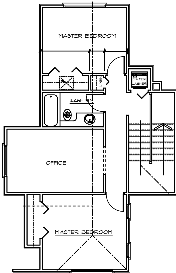
SECOND FLOOR LEVEL 688.00 SQ FT
