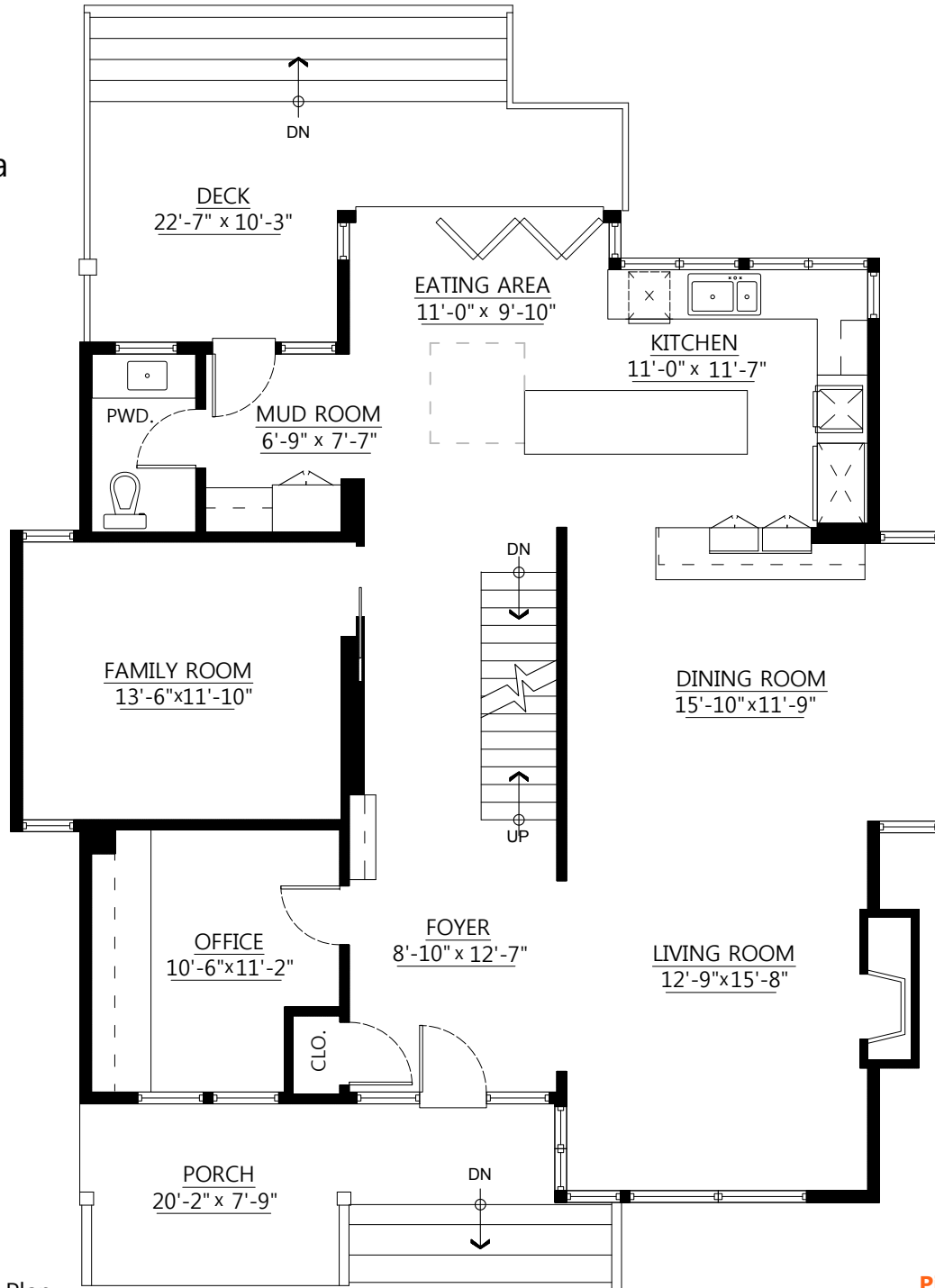
Main Floor Plan Floor Area: 1,337 sq.ft.
