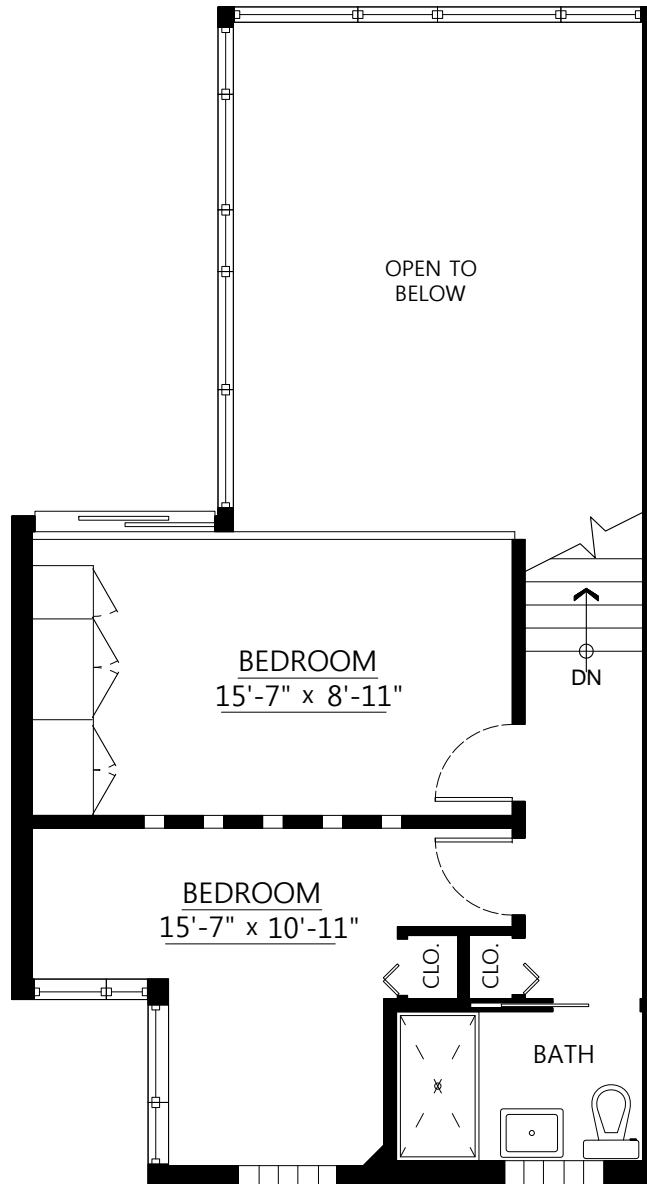
Upper Floor Plan Floor Area: 433 sq.ft.
