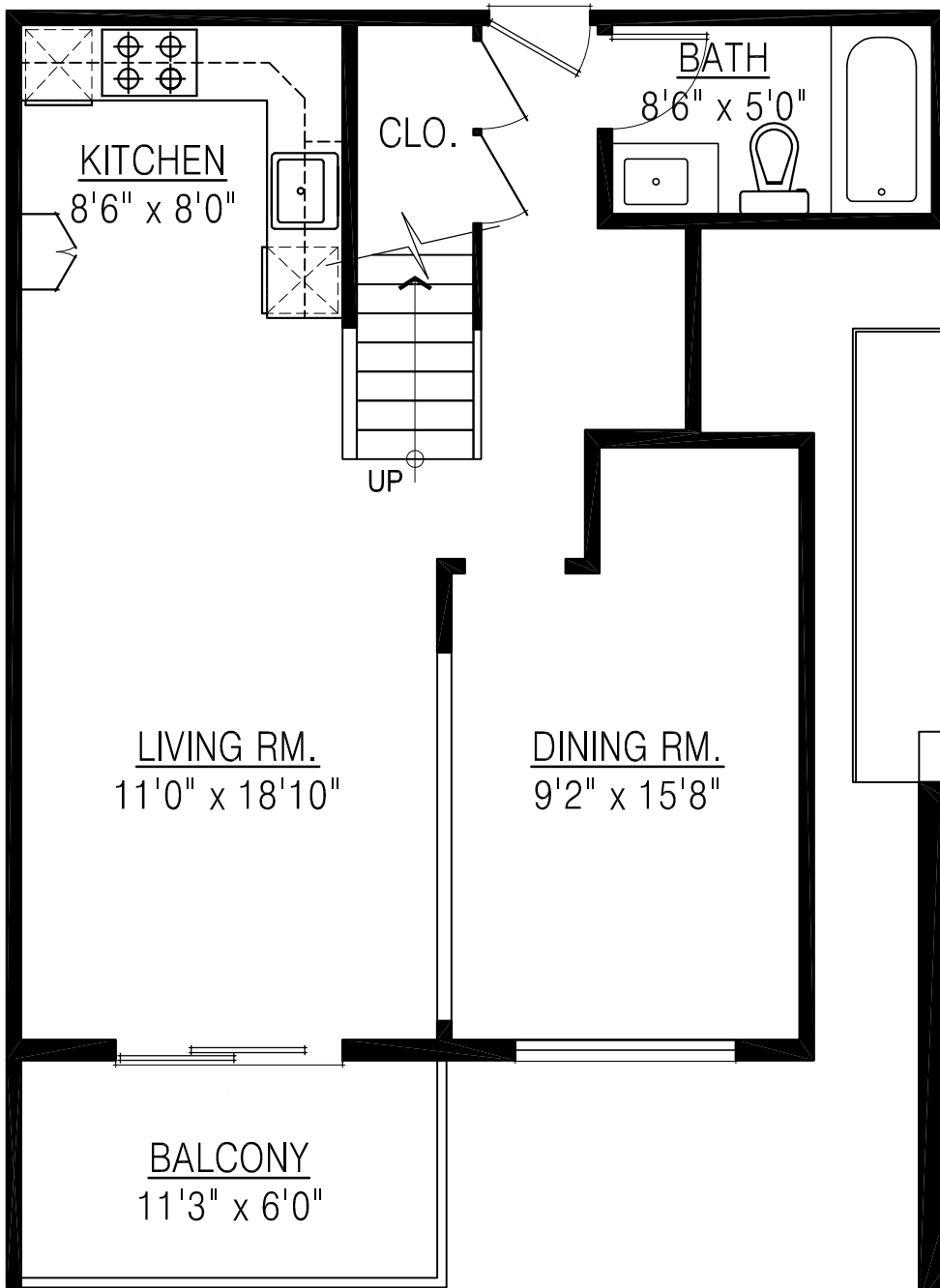
MAIN FLOOR PLAN FLOOR AREA: 596 sq.ft.
