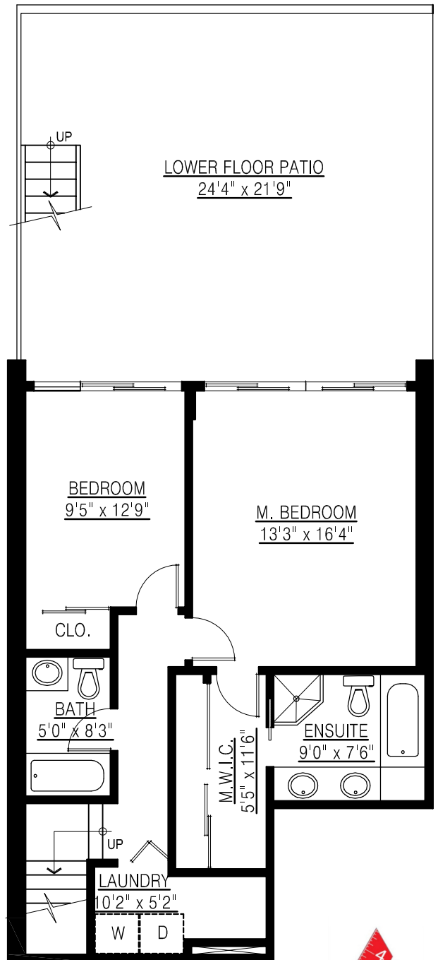
LOWER FLOOR PLAN FLOOR AREA: 732 sq.ft.
