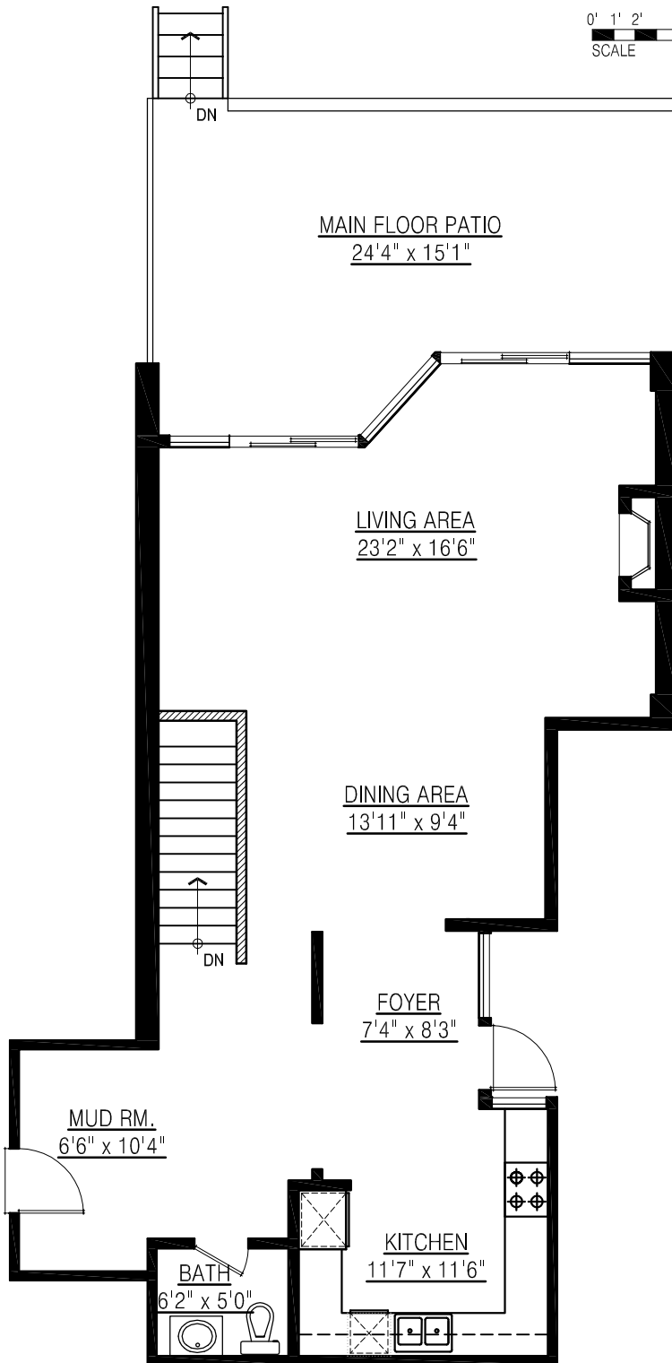
MAIN FLOOR PLAN FLOOR AREA: 990 sq.ft.
