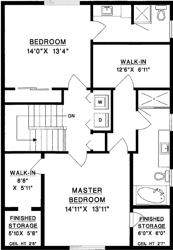
UPPER LEVEL
