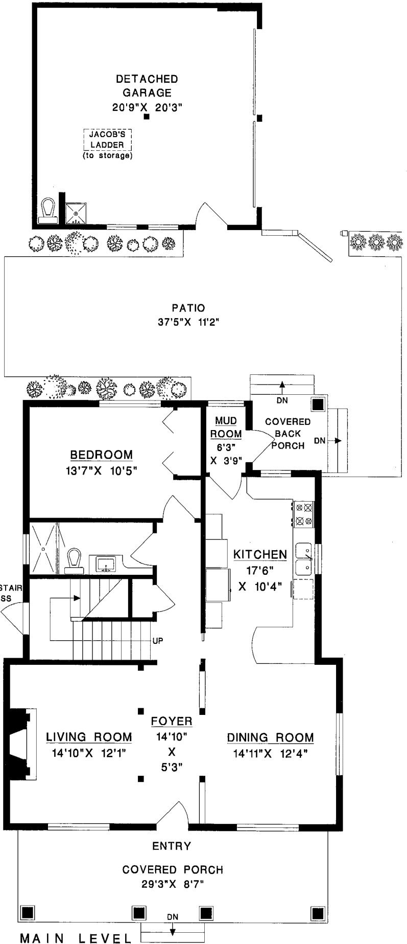
MAIN LEVEL
