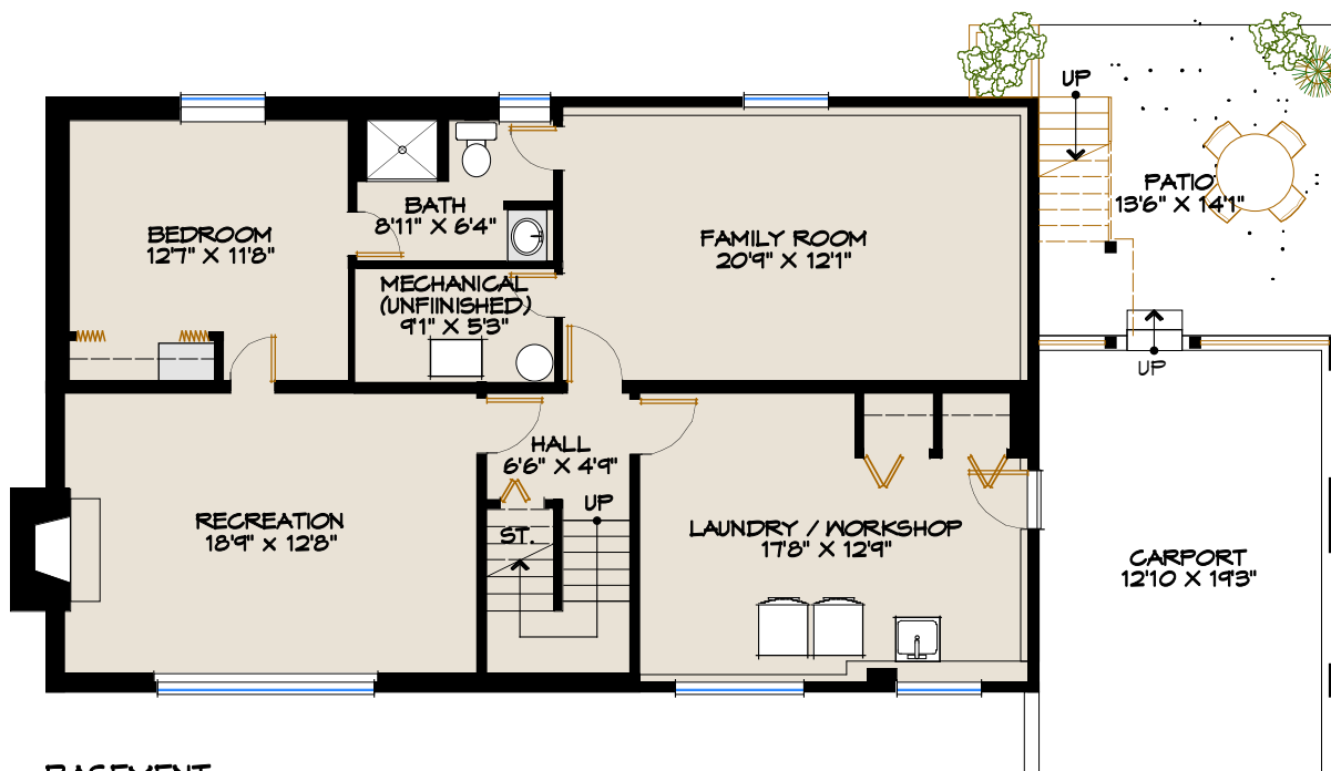
BASEMENT 1162 S.F. FINISHED AREA 46 S.F. UNFINISHED AREA
