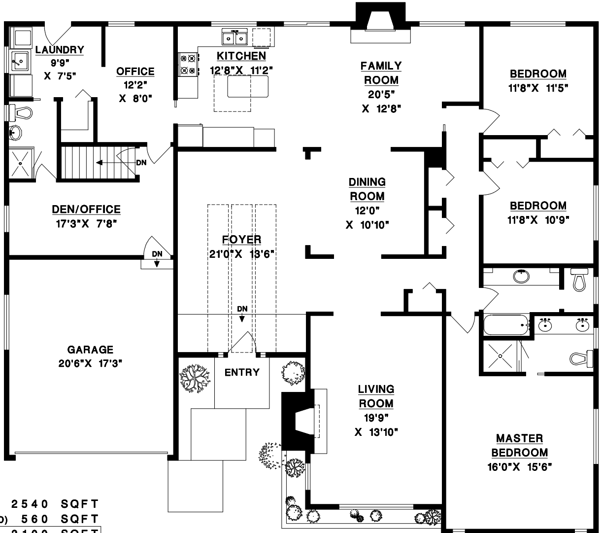
MAIN LEVEL
