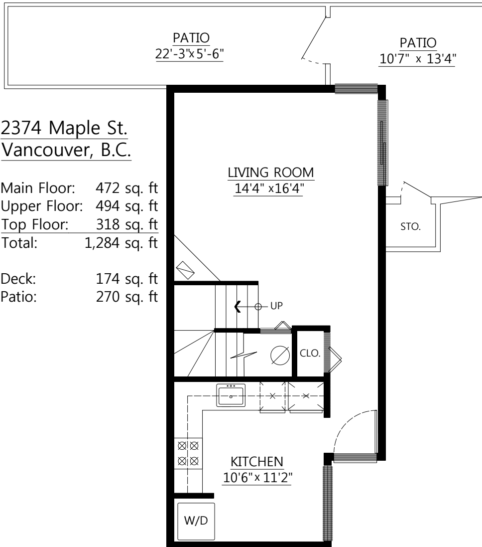
Main Floor Plan Floor Area: 472 sq.ft.
