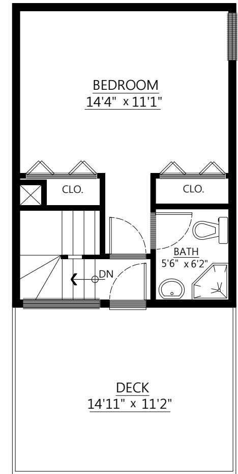
Top Floor Plan Floor Area: 318 sq.ft.
