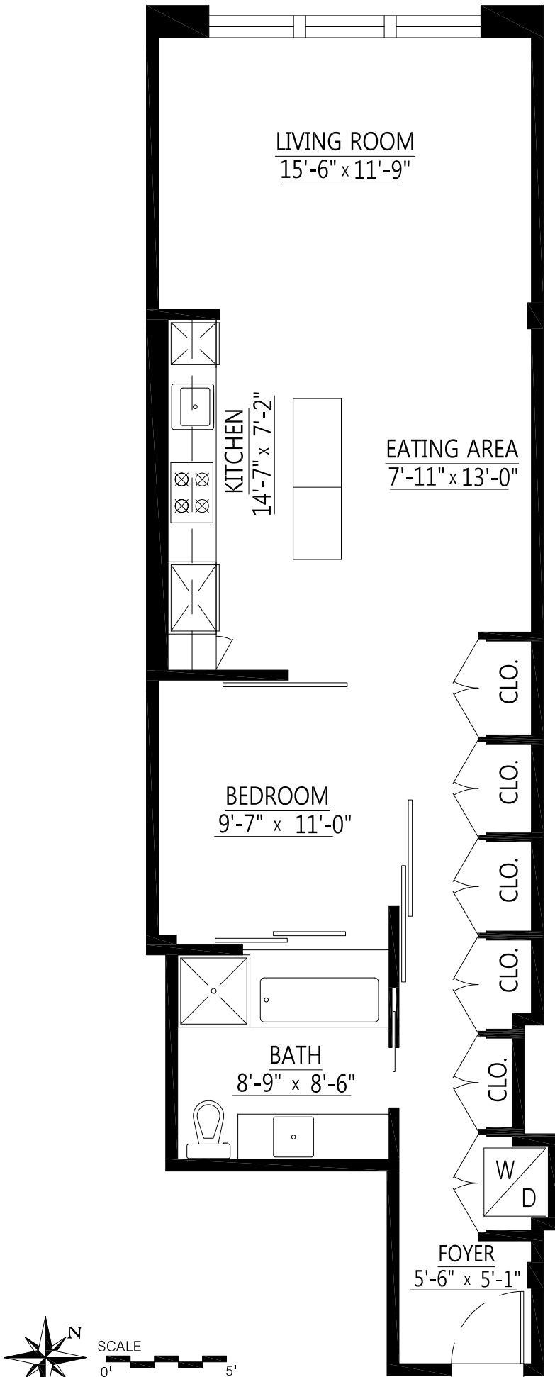
Main Floor Plan Floor Area: 846 sq.ft.
