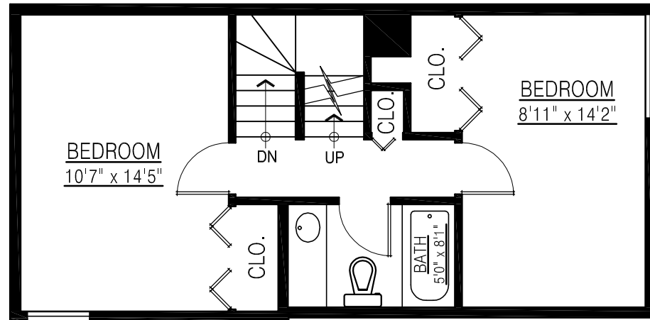
UPPER FLOOR PLAN FLOOR AREA: 478 sq.ft.
