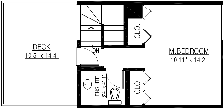
TOP FLOOR PLAN FLOOR AREA: 318 sq.ft.
