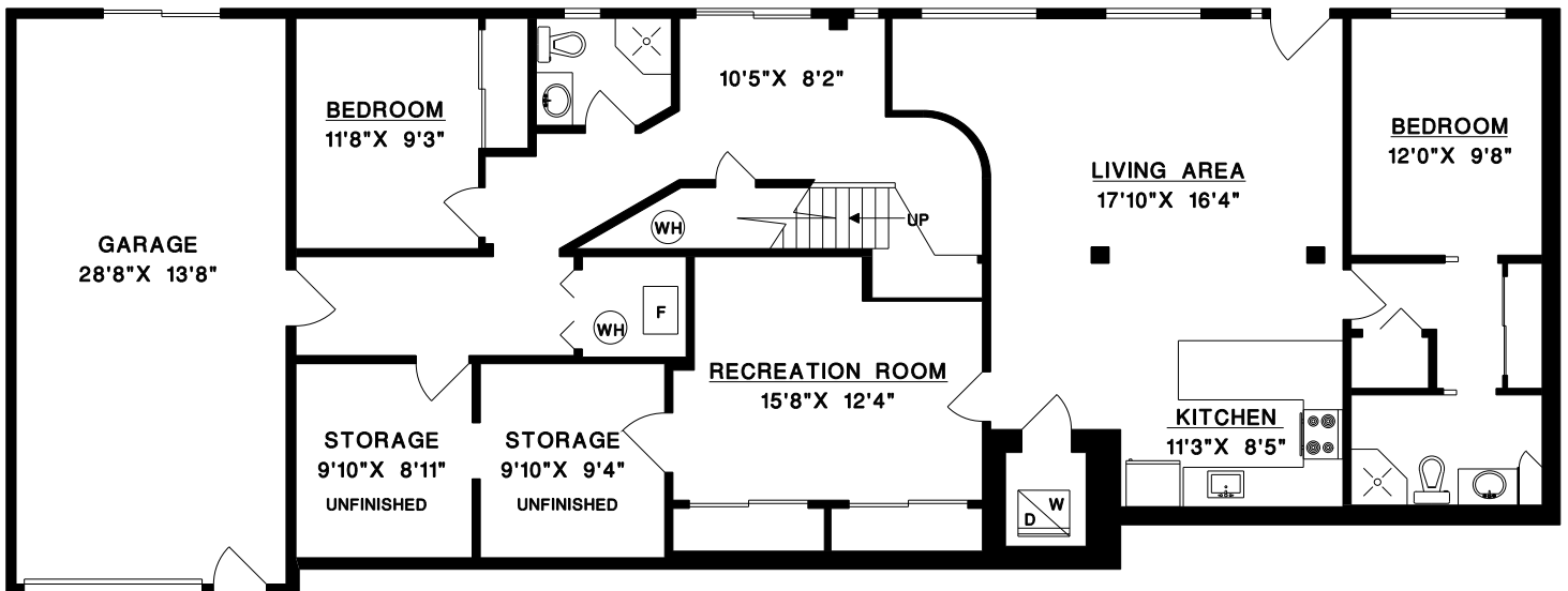
LOWER FLOOR
