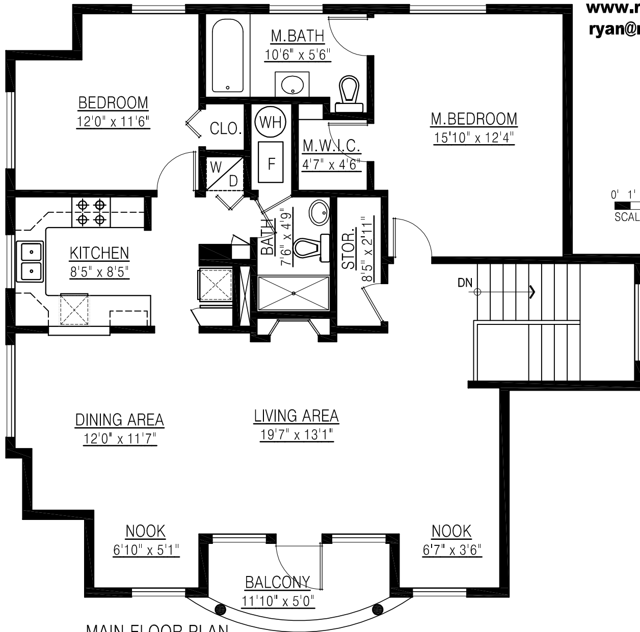
MAIN FLOOR PLAN FLOOR AREA: 1,317 sq.ft.
