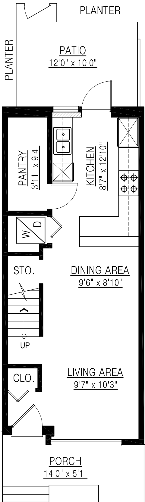
MAIN FLOOR PLAN FLOOR AREA: 464 sq.ft.
