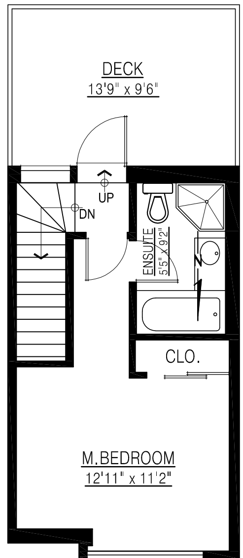
TOP FLOOR PLAN FLOOR AREA: 329 sq.ft.
