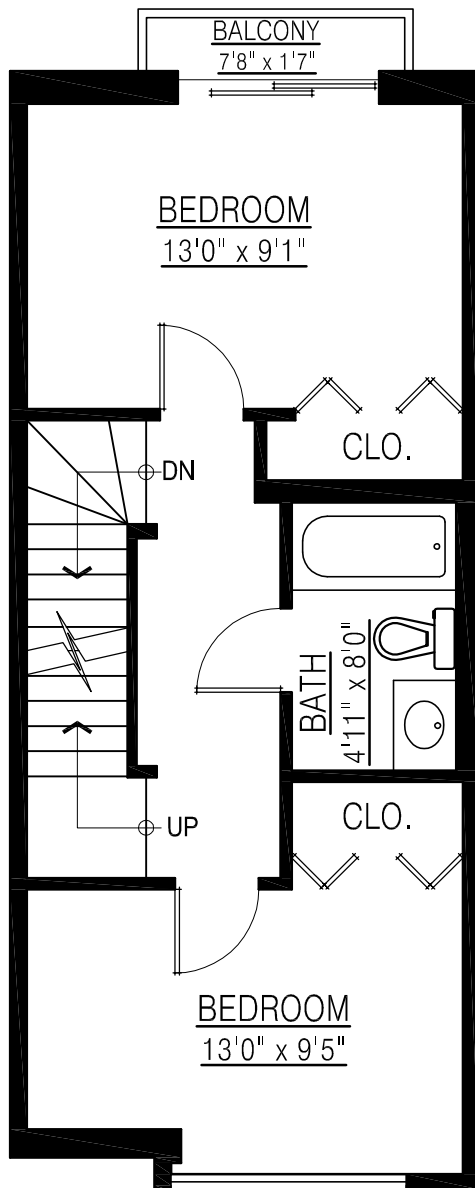
UPPER FLOOR PLAN FLOOR AREA: 464 sq.ft.
