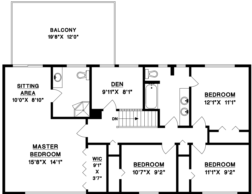
UPPER LEVEL
