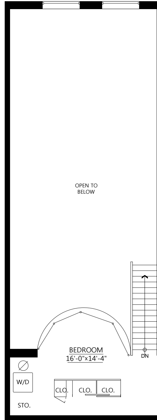
Loft Floor Plan Floor Area: 300 sq.ft.
