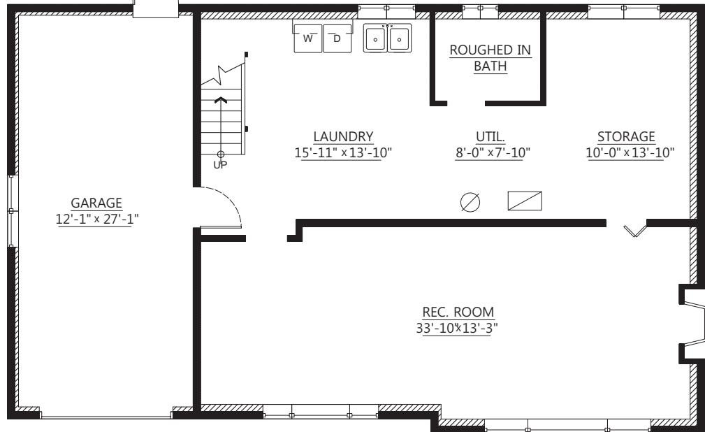
Lower Floor Plan Floor Area: 1,032 sq.ft.
