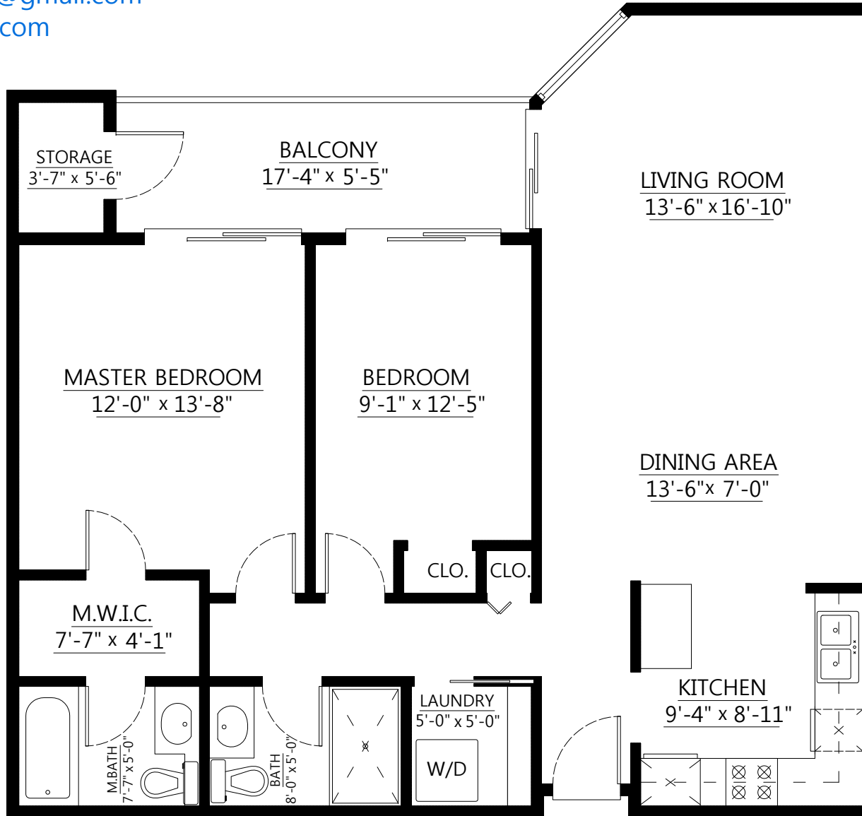
Main Floor Plan Floor Area: 1,019 sq.ft.
