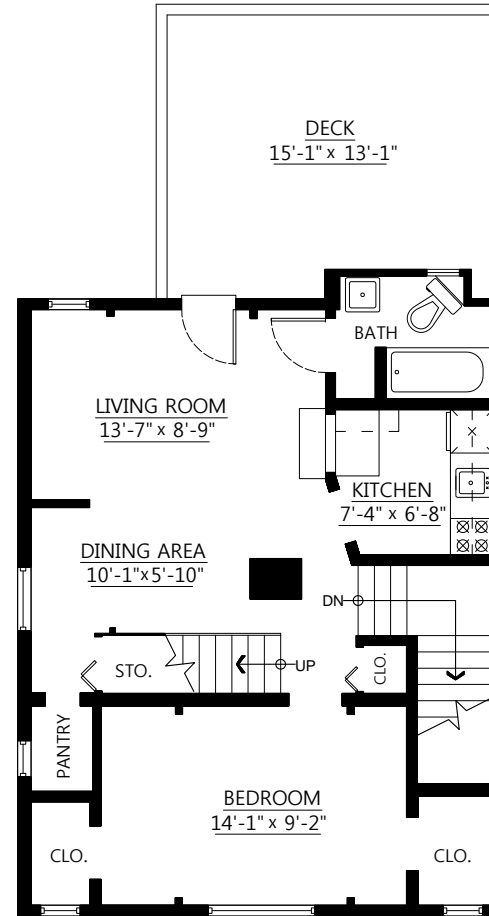
Upper Floor Plan Floor Area: 645 sq.ft.
